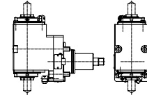
7.073.505 External Coolant • Drilling and Milling Head • Radial, Double Sided • Collet Chuck, ER32 • PRECIFLEX®
